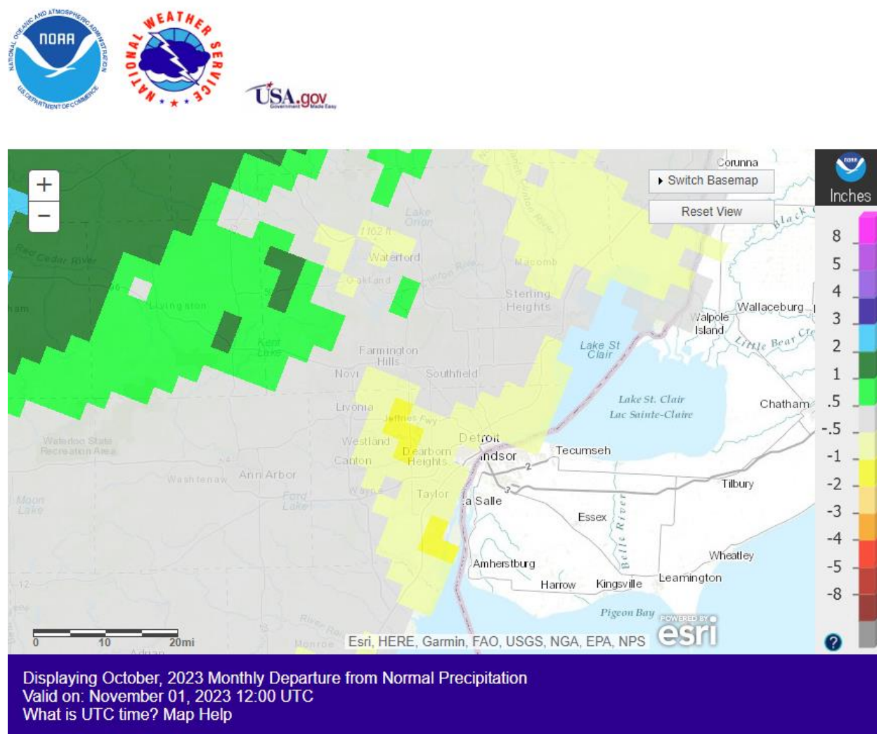
Figure 16: Monthly departure from normal precipitation for the southeastern Lower Peninsula of Michigan for October 2023 from the National Oceanic and Atmospheric Administration.
