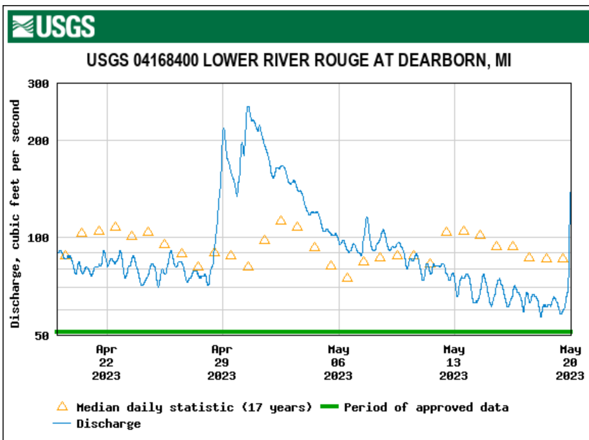
Figure 15: Streamflow data from the United States Geological Survey gage on the Lower Rouge River. Data are shown for the week prior to data collection (April 19, 2023) to the conclusion of all sampling events (May 19, 2023). Seventeen year (17) year median data are depicted by the orange triangles, and the daily mean of stream discharge for the time period under consideration is depicted by the solid blue line.
