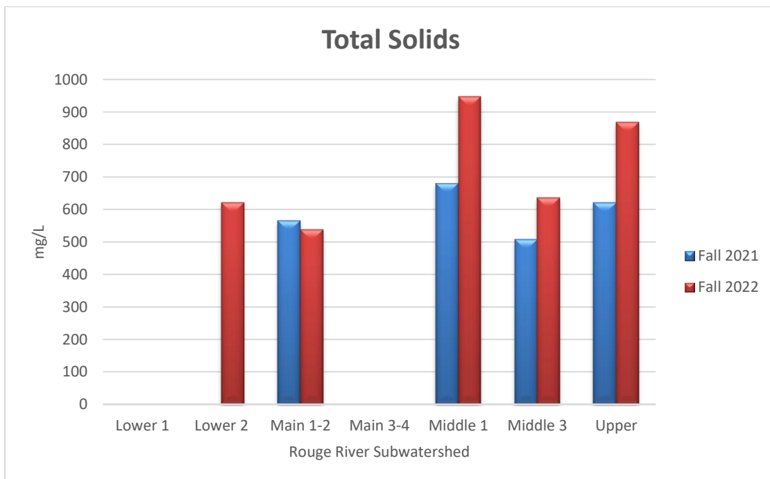
Figure 12: TOTAL SOLIDS results for fall 2021 and 2022. Results were not available for the Lower 1 or Main 3-4 either year, or for the Lower 2 in 2021.
