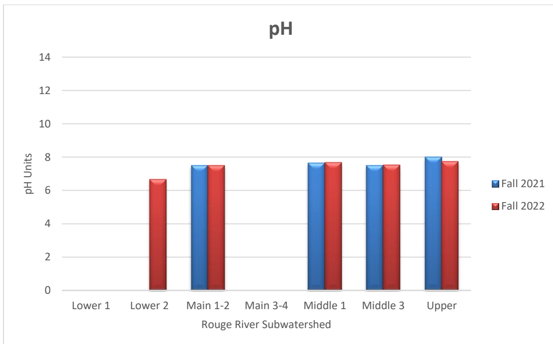
Figure 6: pH results for fall 2021 and 2022 monitoring. Results depict the median value of those collected in each subwatershed. Results were not available for Lower 1 or Main 3-4 either year, or for the Lower 2 in 2021.
