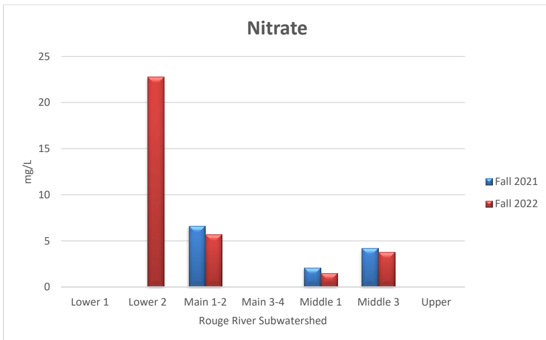
Figure 10: NITRATE results for fall 2021 and 2022 monitoring. Results were not available for Lower 1 or Main 3-4 either year, or for the Lower 2 in 2021. A result of 0 was found for the Upper both years.
