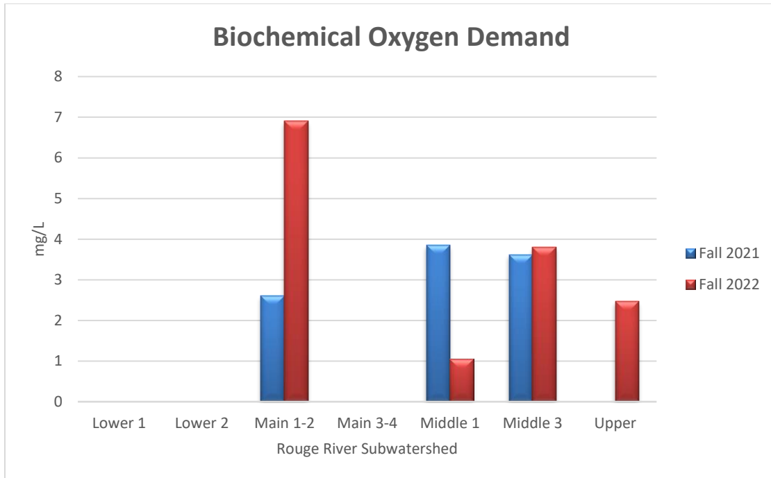
Figure 7: BIOCHEMICAL OXYGEN DEMAND results for fall 2021 and 2022 monitoring. Results were not available for the Lower 1, Lower 2, or Main 3-4 either year, or for the Upper in 2021.
