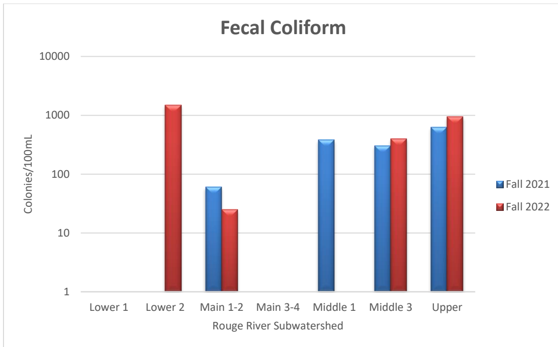
Figure 5: FECAL COLIFORM results for fall 2021 and 2022 monitoring. Results are presented on a logarithmic scale. Results were not available from the Lower 1 or Main 3-4 either year, or for the Lower 2 in 2021 or the Middle 1 in 2022.
