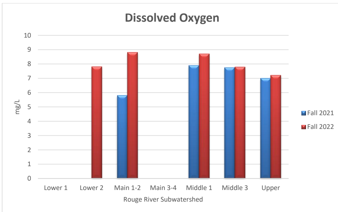
Figure 4: DISSOLVED OXYGEN results from fall 2021 and 2022 monitoring. Results were not available for the Lower 1 or Main 3-4 either year, or for the Lower 2 in Fall 2021.
