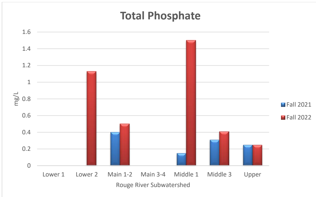
Figure 9: TOTAL PHOSPHATE results for fall 2021 and 2022. Results were not available from the Lower 1 or Main 3-4 either year, or for the Lower 2 in 2021.
