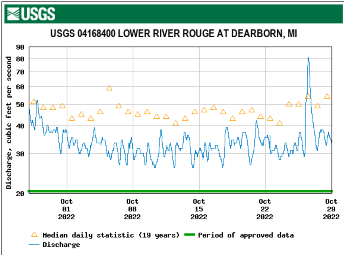
Figure 15: Streamflow data from the United States Geological Survey gage on the Lower Rouge River. Data are shown for the week prior to data collection (September 27, 2022) to the conclusion of all sampling events (October 28, 2022). Nineteen year (19) year median data are depicted by the orange triangles, and the daily mean of stream discharge for the time period under consideration is depicted by the solid blue line.
