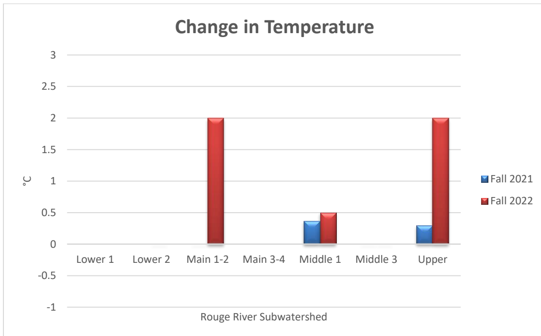
Figure 8: CHANGE IN TEMPERATURE results for fall 2021 and 2022 monitoring. Results were not available for the Lower 1 or Main 3-4 either year, or for the Lower 2 in 2021. Values of 0 were found for the Main 1-2, and Middle 3 in 2021, and the Lower 2 and Middle 3 in 2022.
